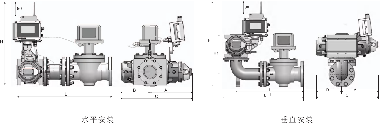
图5-8 G□/TFC-□/TCVL-B-□-R
