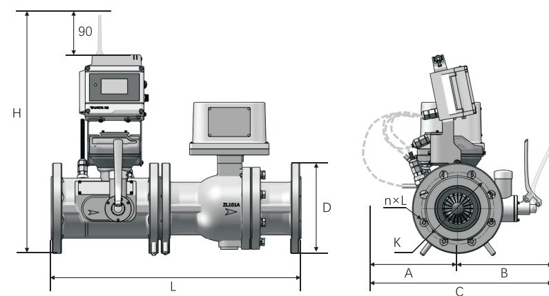
图3-11 TBQM-□/TFC-□/TCVL-M
