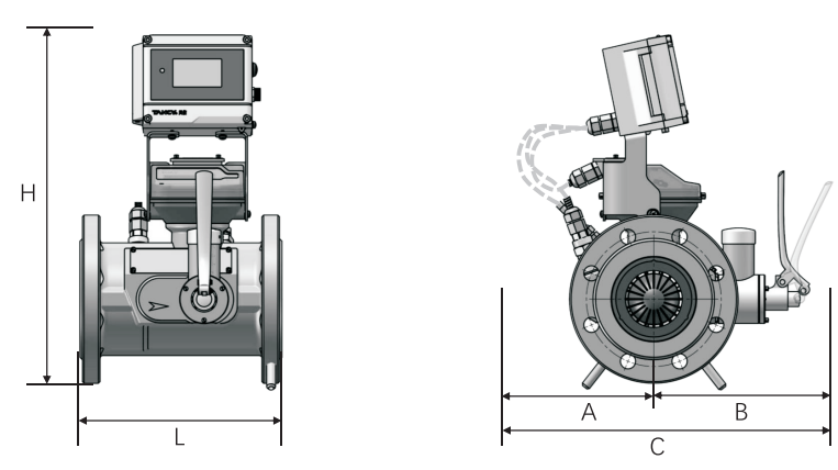
图3-4 TBQM-□/FCM-V
