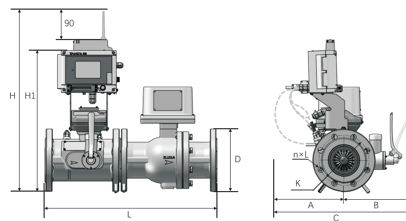
图3-7 TBQM-□/FCF-III-□-M
