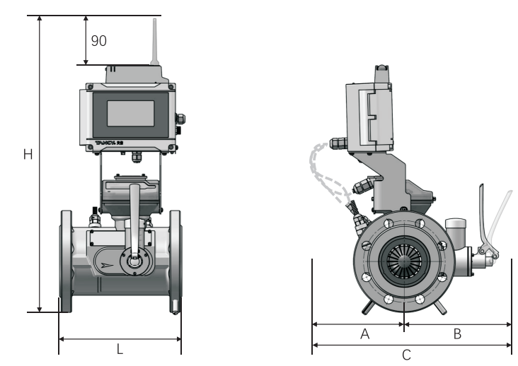
图3-3 TBQM-□/TFC-B
