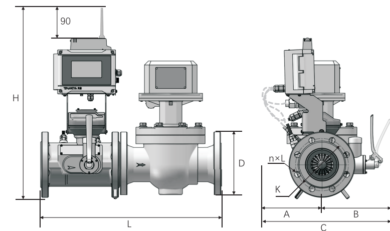
图3-10 TBQM-□/TFC-□/TCVL-B
