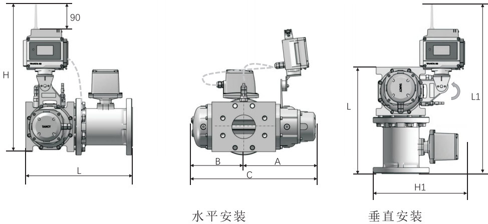
图5-8 TEP-G□-1
