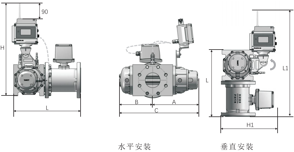
图5-13 TYLZ-G□-N/TCVL-C-□-R
