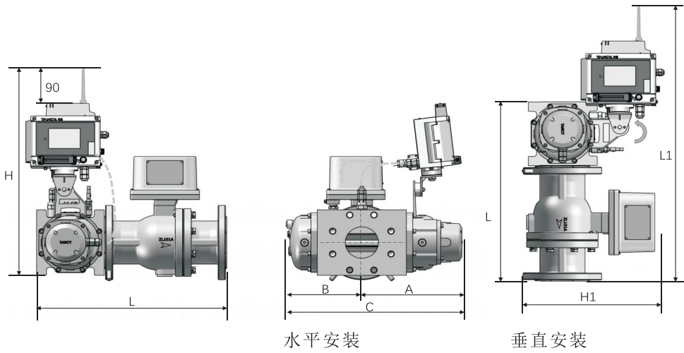
图5-7 TYL-G□C-□-M
